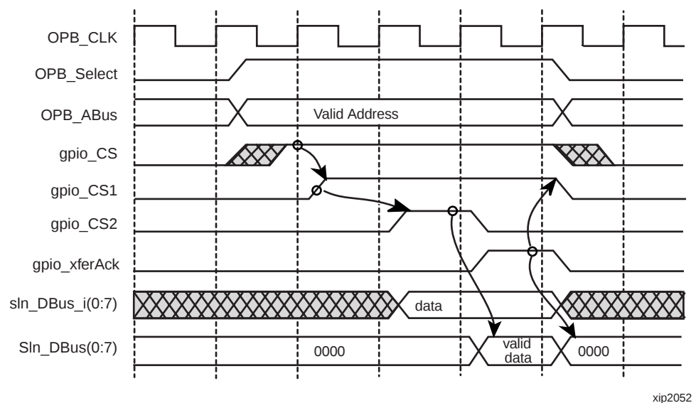
Figure 12: Timing Diagram for the OPB Slave Interface
