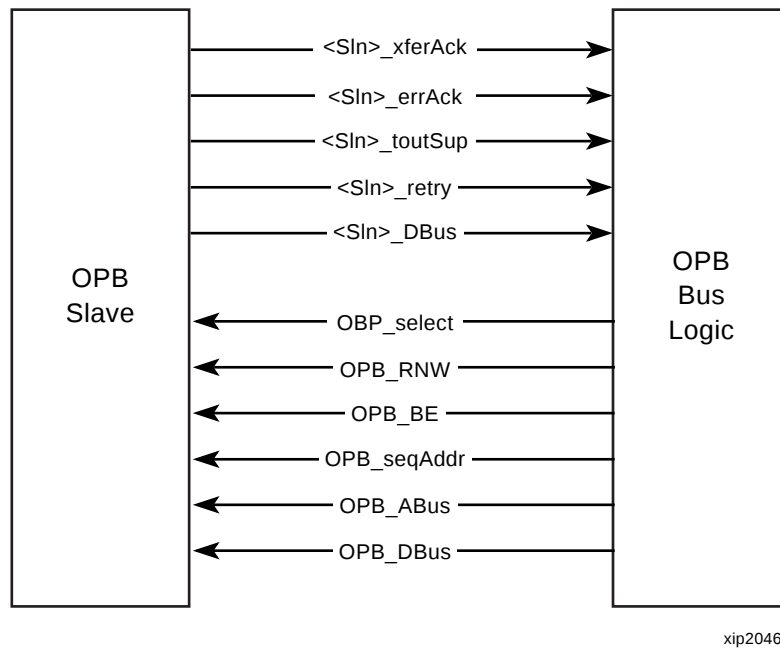
Figure 4: OPB Slave Interface
