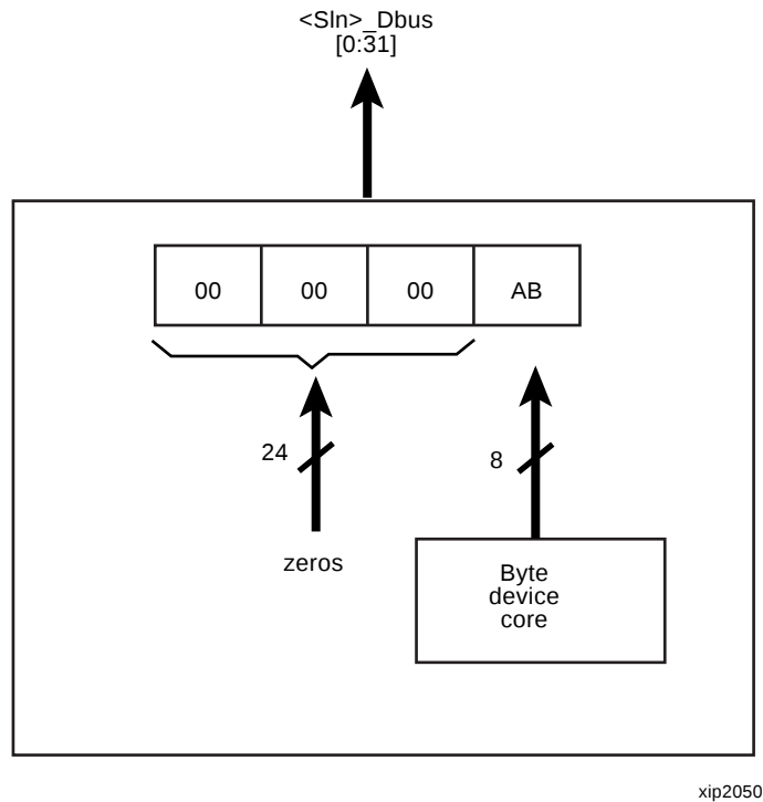
Figure 8: Expand a Byte Device to 32 Bits Wide
