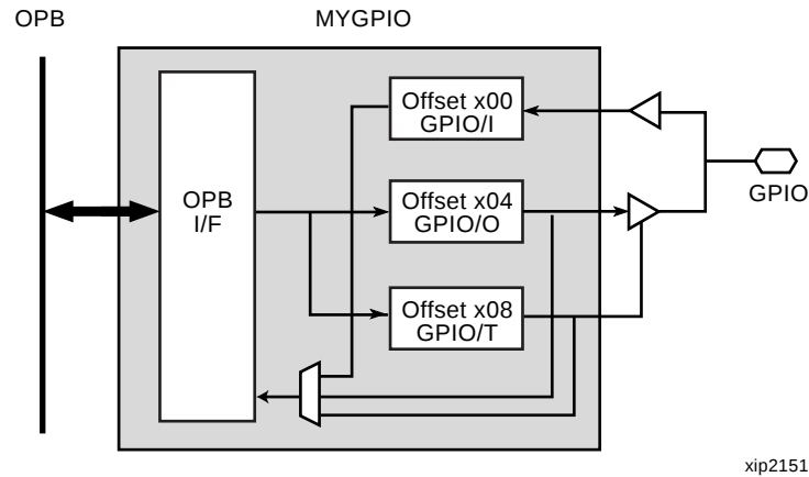
Figure 9: Block Diagram for MYGPIO
