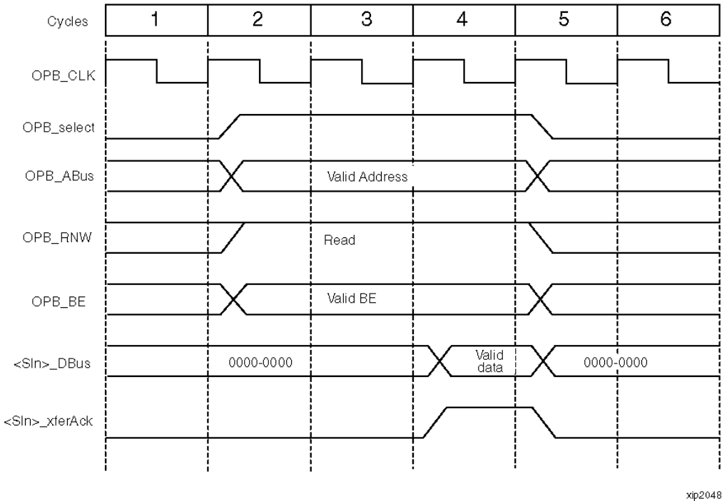
Figure 6: A Basic OPB Read Transaction (Example)
