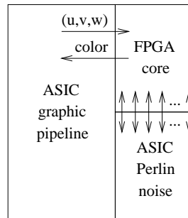
Figure 15: ASIC+FPGA Procedural Texture Mapping Organization
