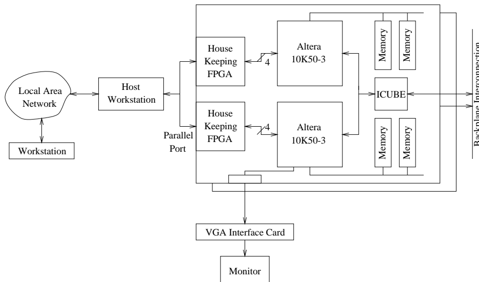
Figure 2: Experimental Setup
