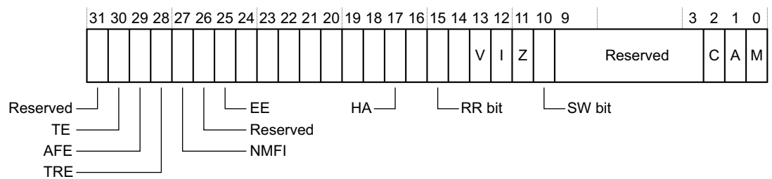
Figure 4-8 SCTLR bit assignments
