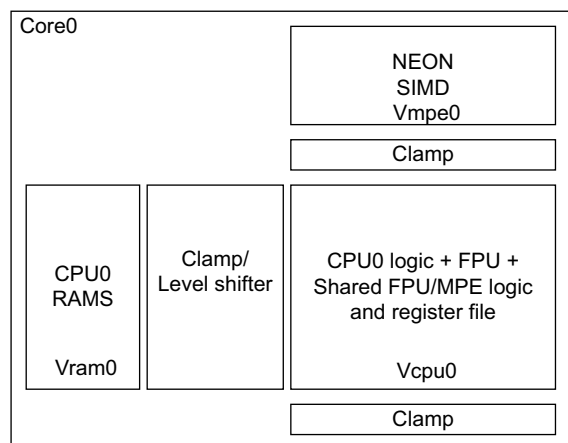
Figure 2-4 Power domains for the Cortex-A9 processor
