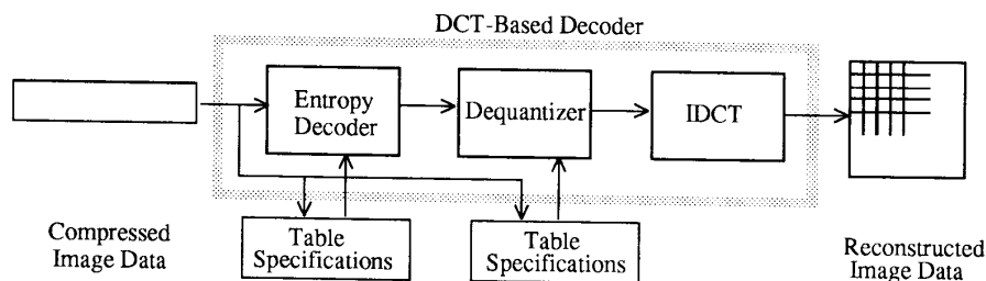
Figure 2. DCT-Based Decoder Processing Steps
