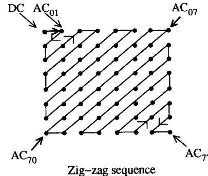
Figure 3. Preparation of Quantized Coefficients for Entropy Coding
