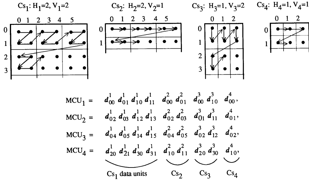
Figure 8. Generalized Interleaved Data Ordering Example
