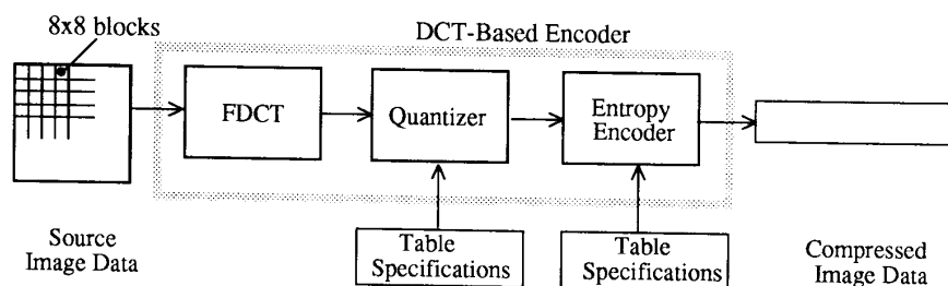
Figure 1. DCT-Based Encoder Processing Steps
