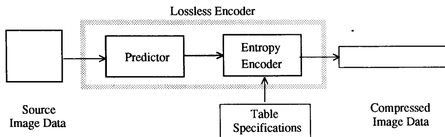
Figure 4. Lossless Mode Encoder Processing Steps
